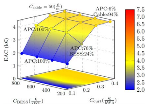
Most economic grid expansion strategy for an exemplarily low voltage grid
