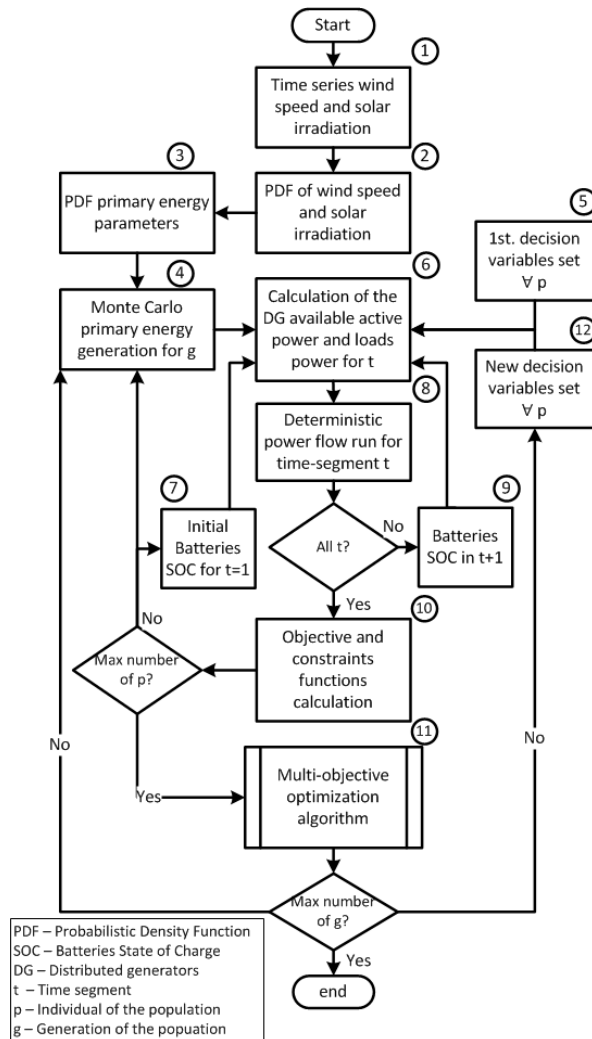
Microgrids planning methodology
